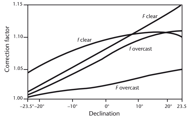
Comparison of calculated and empirically determined correction factors for a shading ring, with b/r = 0.169 ; f indicates calculated curves and F indicates empirical ones (after Dehne, 1980).
